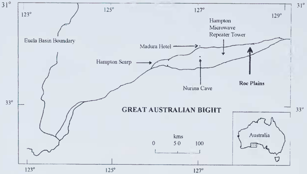
Figure 1 Locality map for the Roe Calcarenite and the Hampton Microwave Repeater tower.
